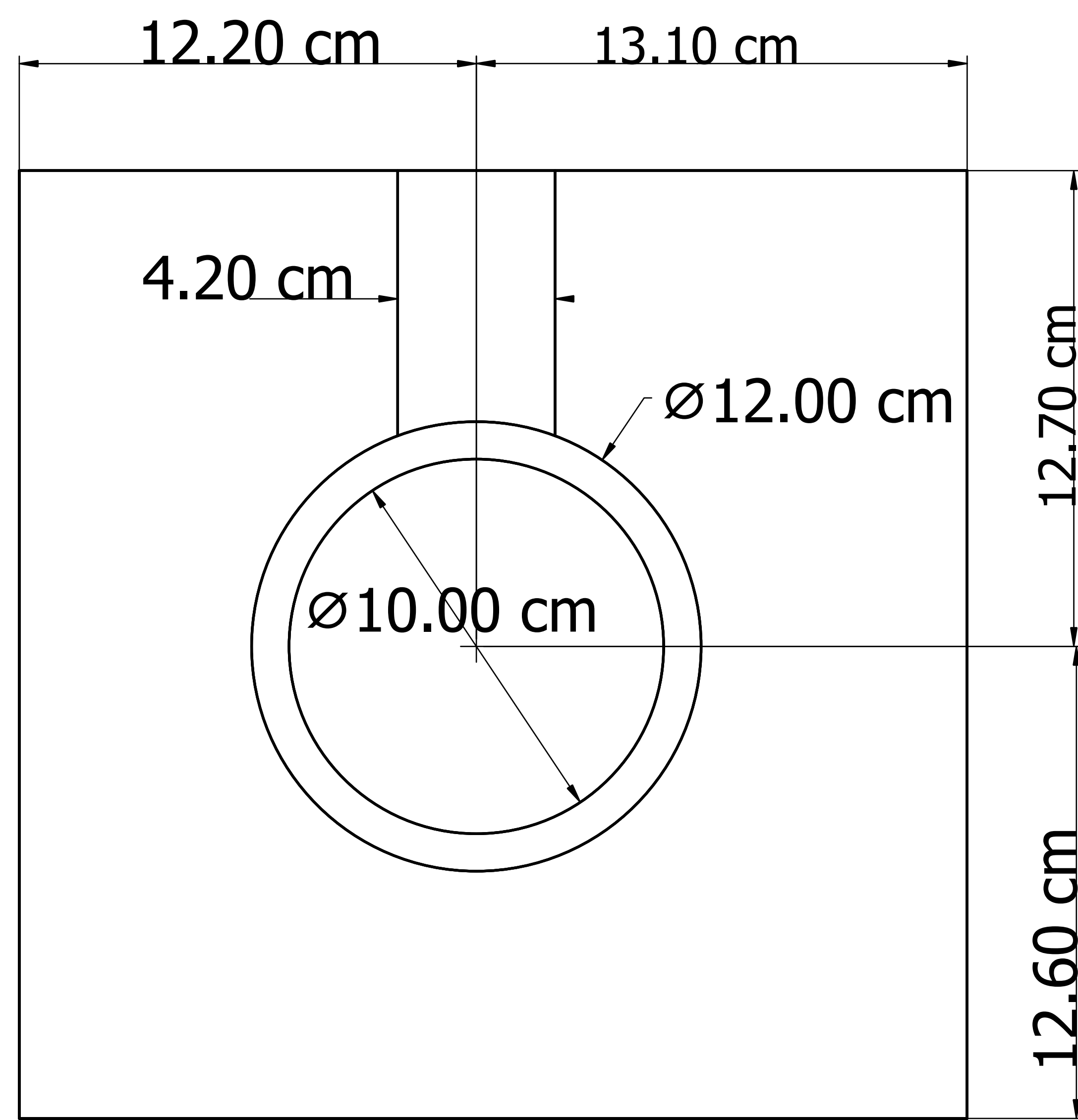
Top View
