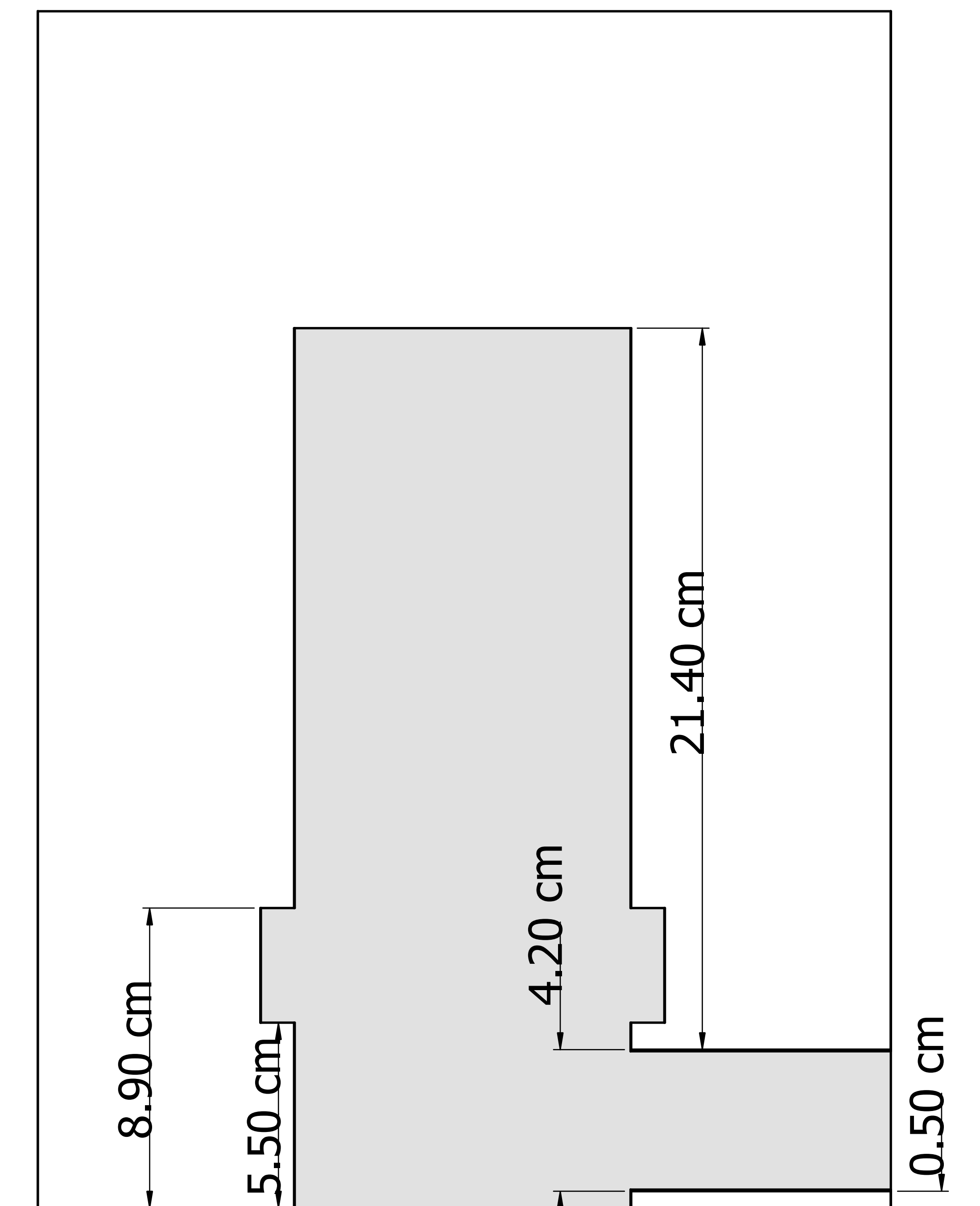
Side View-Cross Section
