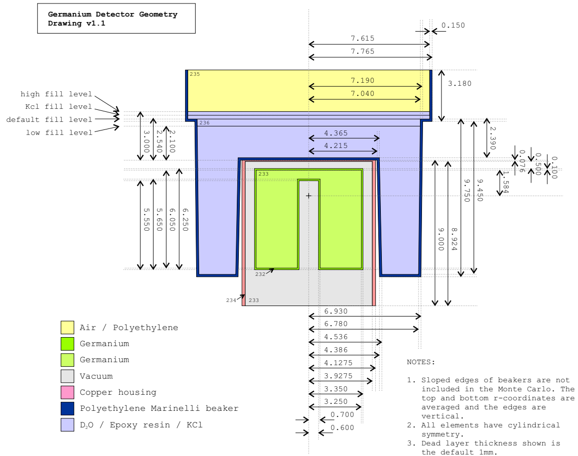
Figure 2: The Ge detector geometry, as implemented in SNOMAN.
