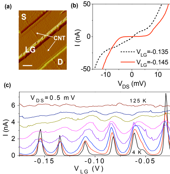
Figure 2: (Color online) Device A: (a) Tapping mode atomic force micrograph with 100 nm wide Al local gate (LG) and Pd source (S) and drain (D) top contacts (scale bar is 200 nm). (b) I - V_{DS} curves at two different gate voltages at 4.2 K, showing Coulomb Blockade and single electron tunneling. (c) Current versus local gate voltage showing several reproducible peaks for several temperatures (bottom to top: 4.2, 12, 20, 35, 50, 75, 100, and 125 K). Peaks begin to wash out around 125 K, for which k_B T \sim 11 meV.
