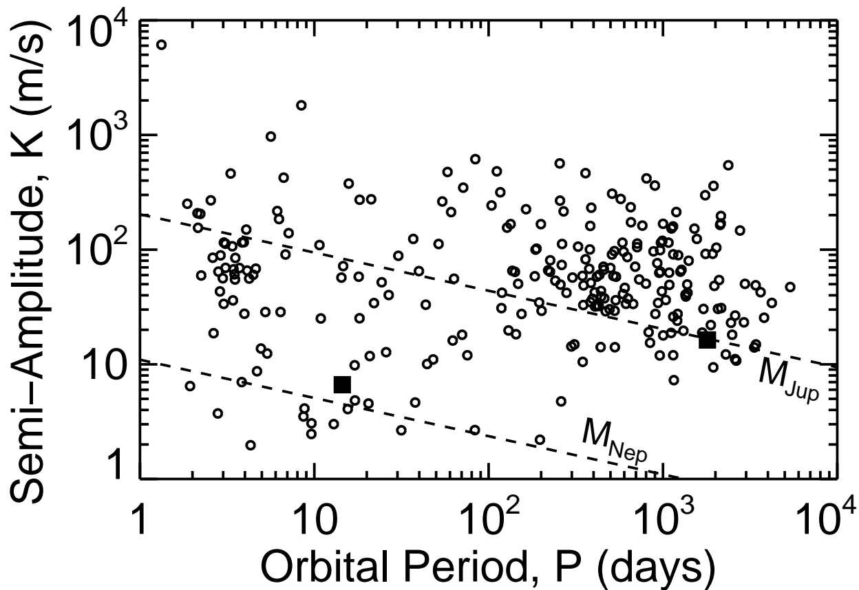
Fig. 8.— Velocity semi-amplitude vs. orbital period for planets with radial velocity detections. The two planets announced in this paper are indicated by filled squares. Diagonal dashed lines show the approximate locus of Jupiter and Neptune mass planets, assuming M = M_{\odot} , e = 1 , and \sin i = 1 . Detecting low mass planets with long periods is particularly challenging.
