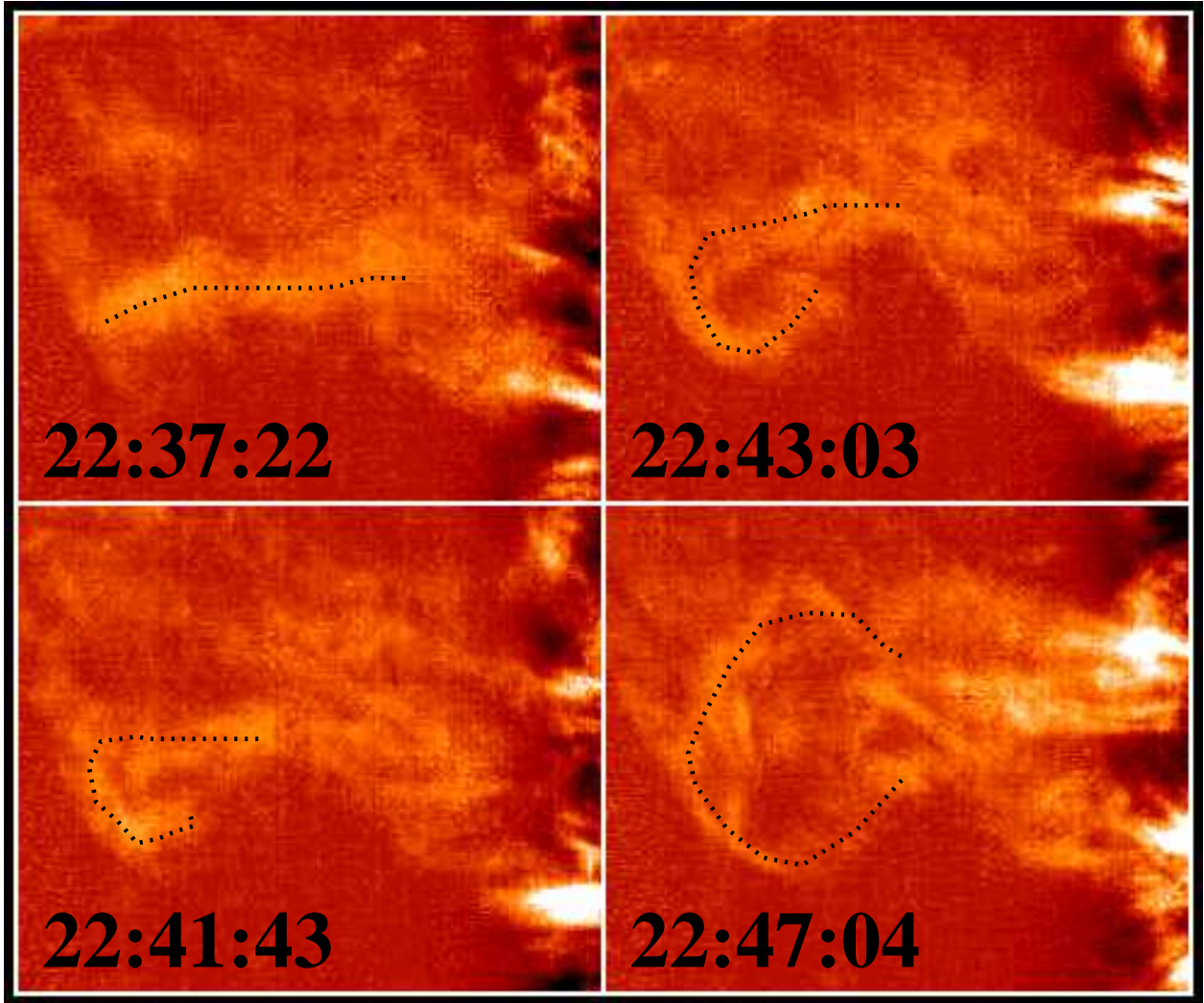
Fig. 6.— Time sequence of the Ca II filtergrams (see the black dotted window in the right panel of Fig. 1) showing the cyclone-like motion of plasma. The FOV is about 26.4'' \times 22'' . The curves are described in the text.
