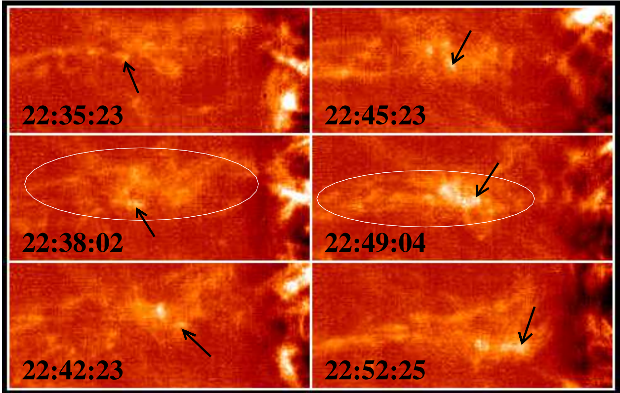
Fig. 5.— Time sequence of the Ca II filtergrams (see the dash-dotted window in the right panel of Fig. 1) showing the evolution of waterfall-like plasma. The FOV is about 26.4'' \times 11'' . The arrows and two ellipses are described in the text.
