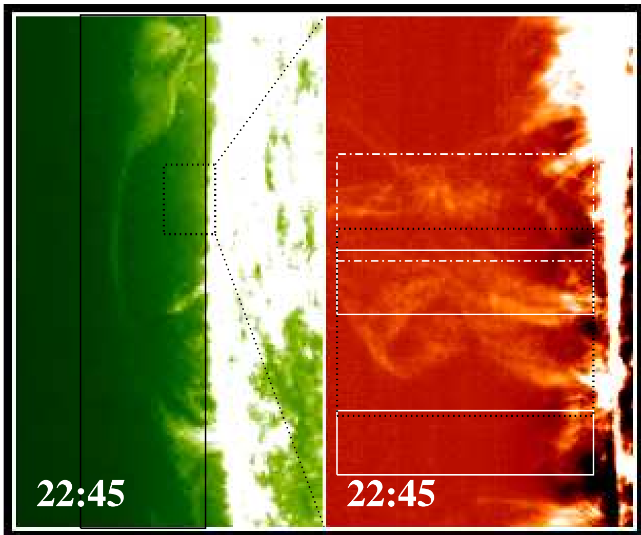
Fig. 1.— An EUV 304 Å image ( left ) from EUVI on STEREO and a Ca II image ( right ) from SOT aboard Hinode on 2007 May 10. On the EUV 304 Å image, the larger box encloses an arch (see Fig. 2), and the smaller box underneath the arch, outlines the field-of-view (FOV) of the right Ca II filtergram. The two solid rectangle windows on the Ca II image denote sub-areas where individual dynamic structures flow downward from corona to chromosphere (see details in Fig. 3), the dash-dotted window, the area where plasma shows waterfall-like motion (see also Fig. 5), and the dotted window, the region in which plasma displays cyclone-like motion (see Fig. 6). The FOV for the EUVI image is about 238'' \times 397'' , and 33'' \times 55'' for the SOT Ca II filtergram.
