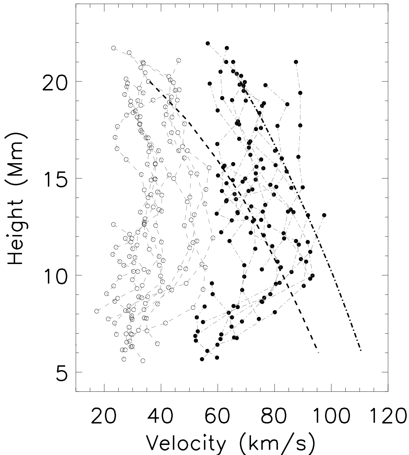
Fig. 4.— Relationship between the downflow velocities of the dynamic structures and the height to the solar surface. The solid circles and the hollow circles denote the velocities of the two types of dynamic structures (see the text), respectively. The individual trajectories (the dash-dotted curves connecting the solid circles, and dashed curves the hollow circles) of the 26 dynamic structures are plotted. The two heavy curves representing the free-fall tracks are fitted to the observed falling velocities at the heights where the bright dynamic
