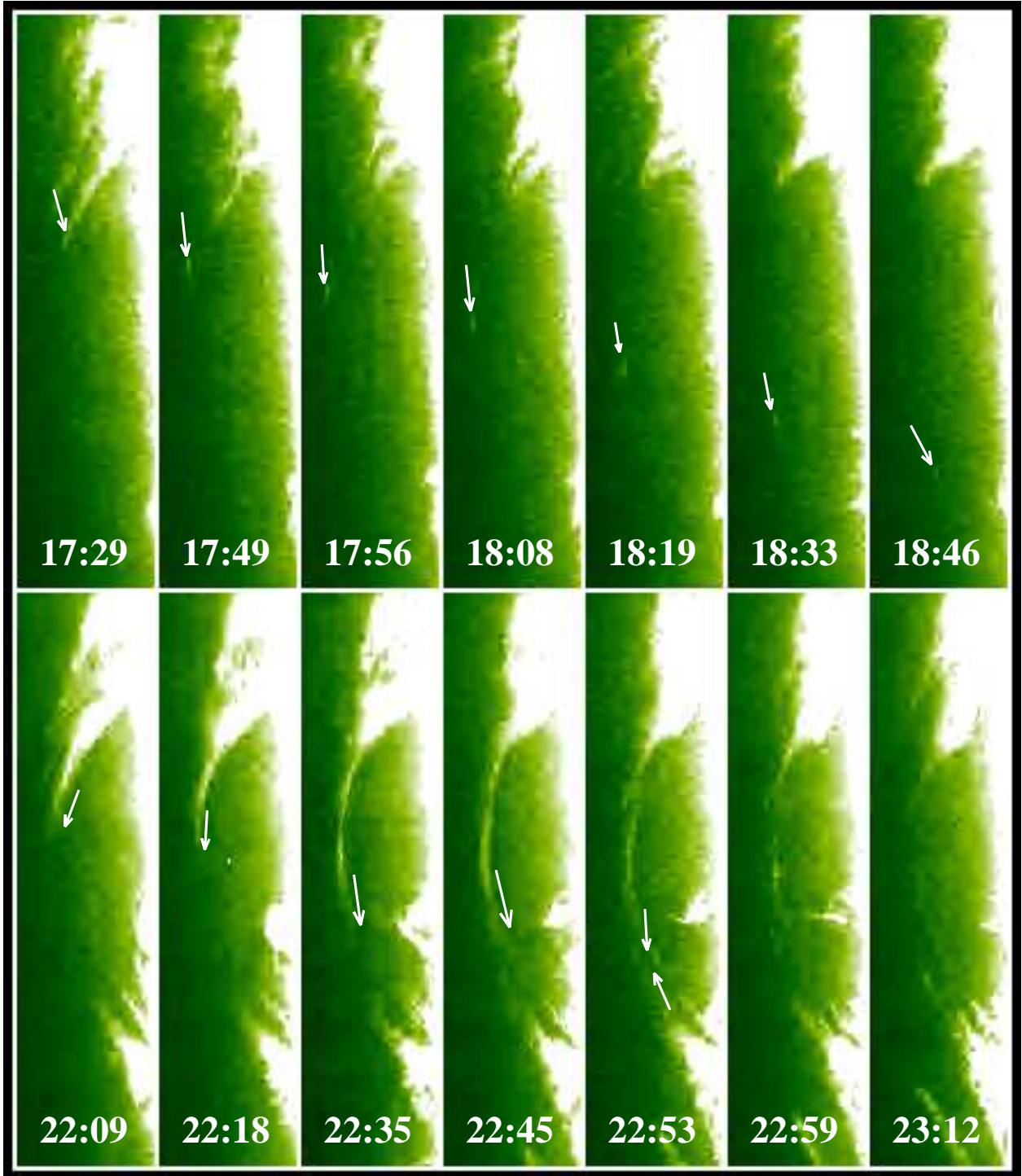
Fig. 2.— Time sequence of the EUV 304 Å images (see the larger rectangle window in the left panel of Fig. 1) showing the dynamics of the arch. The arrows are described in the text. The FOV is about 95'' \times 397'' .
