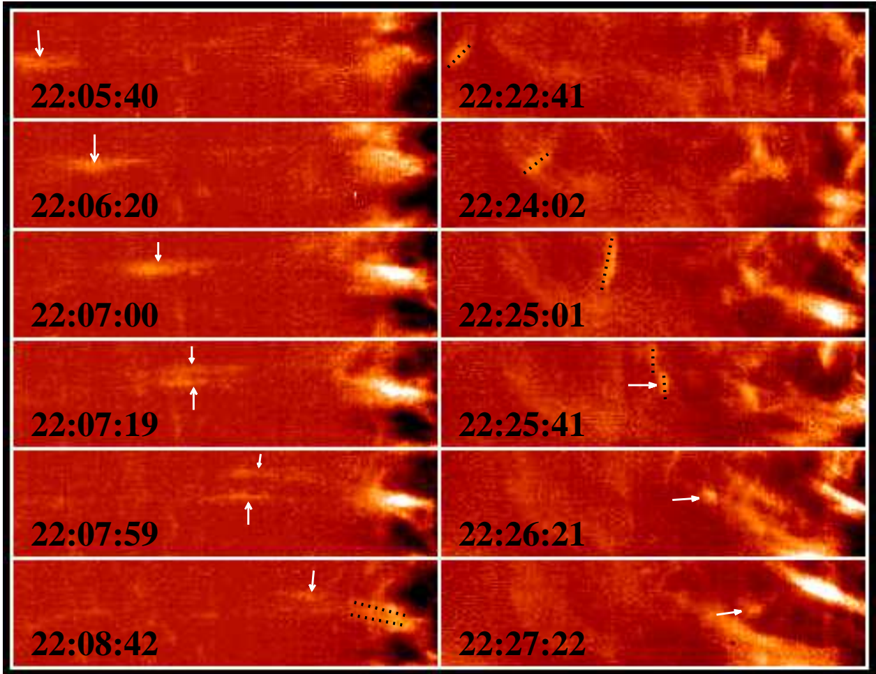
Fig. 3.— Time sequence of the Ca II filtergrams showing the evolution of two dynamic structures. The left column corresponds to the region of the lower solid rectangle window in the right panel of Fig. 1, and the right column to the region of the upper solid rectangle window. The FOV is about 26.4'' \times 6.6'' . The arrows and dotted lines are described in the text.
