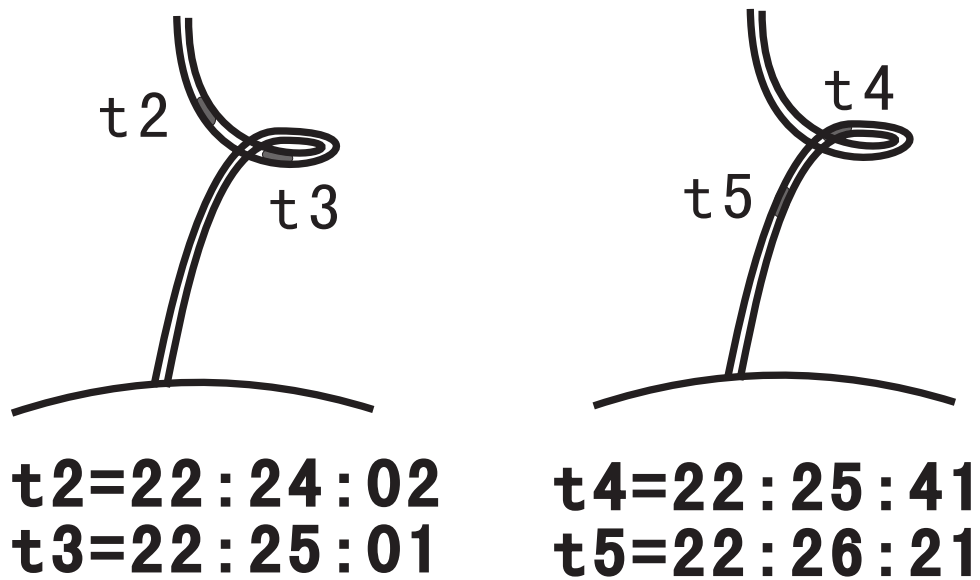
Fig. 7.— The schematic diagrams illustrating the evolution of the type I dynamic coronal structures at t_0 and t_1 (a), and type II dynamic coronal structures at t_2 , t_3 , t_4 , and t_5 (b), respectively. t_0 , t_1 , t_2 , t_3 , t_4 , and t_5 are the observational times displayed in Fig. 3. The solid lines represent the magnetic field lines, as well as the solid points, the dynamic coronal structures.
